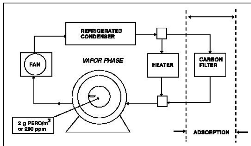
Figure 1. Vapor phase of the "4th and 5th Generation" dry-cleaning machines. The large, regenerable, carbon filter is used to reduce concentrations in the drum below approximately 300 ppm during the final phase of the dry cycle.
